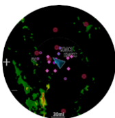
RADAR NEXRAD
